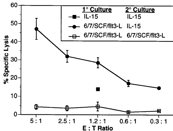
Figure 1. Lytic activity of Lin^- , c-kit^+ , Sca2^+ cells cultured with a cocktail of early acting cytokines \pm IL-15. Sorted cells were cultured in the indicated cytokines as described in Materials and Methods. Cytotoxic activity was assessed on YAC-1 tumor cells. The data are representative of six experiments.
