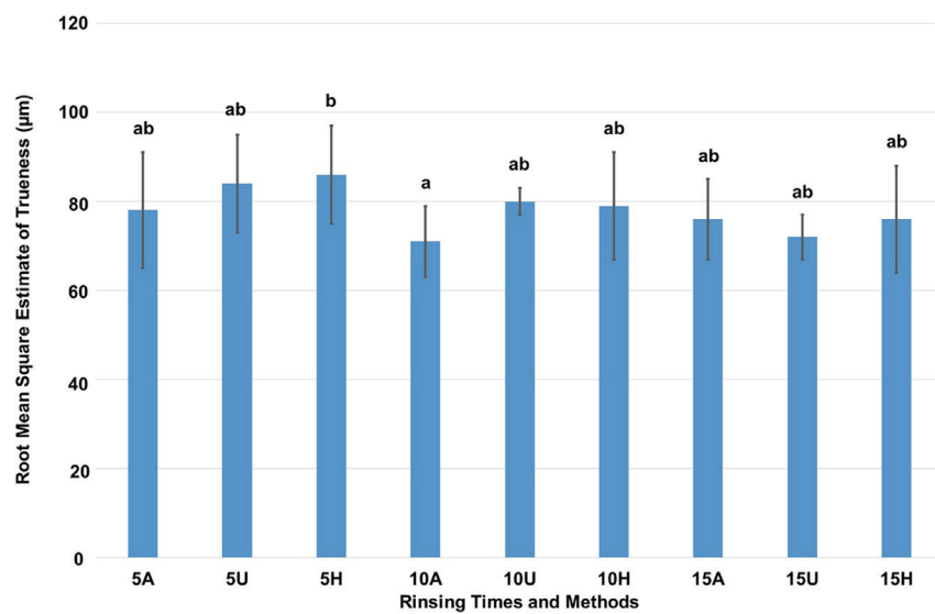
Fig. 5. Mean of RMSE values of trueness obtained for different rinsing times and methods. Different letters indicate significant differences among groups ( P < .05 ). Numbers 5, 10, and 15 denote rinsing times of 5, 10, and 15 min, respectively. Letters A, U, and H stand for automated, ultrasonic, and hand washing, respectively.
