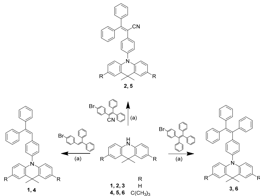
Scheme 1. Syntheses scheme of compounds 1–6. (a) NaOt-Bu, Pd(OAc) 3 , P( t -Bu) 3 , anhydrous toluene, reflux.
