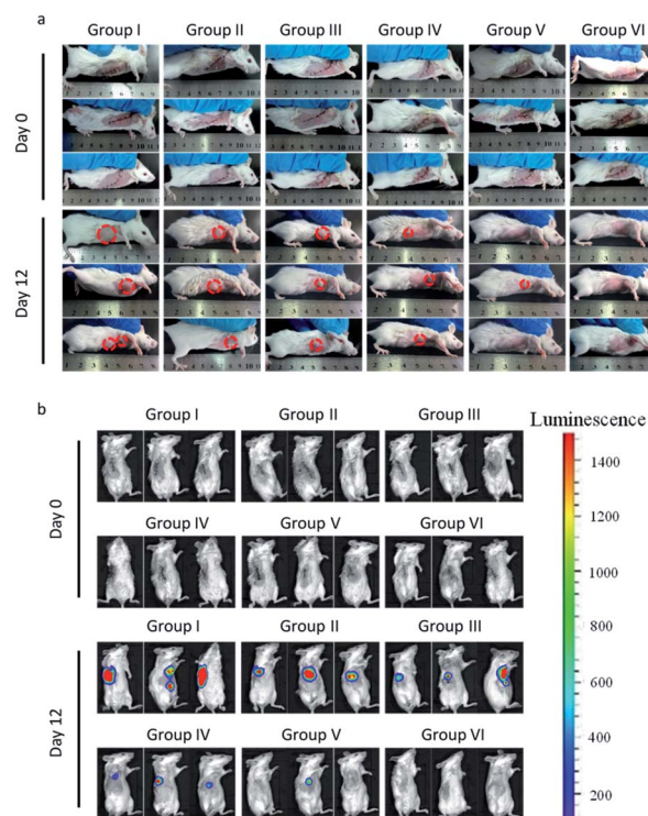
Fig. 6 In vivo tumor immunotherapy to reduce post-surgical tumor relapse by CaIPC. Photographs of mice (a) and in vivo bioluminescence images of the 4T1-Luc tumors (b) of different groups after the removal of the primary tumor (group I, NS; II, CaP; III, CaIP; IV, CaPC; V, LIPC; and VI, CaIPC), and various treatments are indicated. The injected doses of IDOi and CpG ODNs were respectively 600 \mu g kg -1 and 500 \mu g kg -1 each time.
