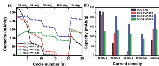
Fig. 11 (a) Rate cycling performance for the samples measured at varying current densities from 10 to 100 mA g -1 . (b) Average discharge capacities of the samples measured at 10, 20, 50, 100, and 10 mA g -1 .
