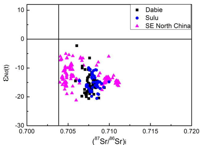
Figure 3 | Initial ^{87}Sr/^{86}Sr ratios vs. \epsilon_{Nd}(t) values for postcollisional mafic igneous rocks in east-central China.
