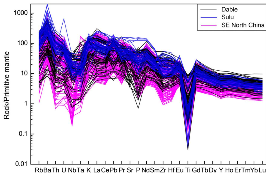
Figure 2 | Primitive mantle-normalized trace element patterns for postcollisional mafic igneous rocks in east-central China. The primitive mantle trace element contents are from Ref. 36.
