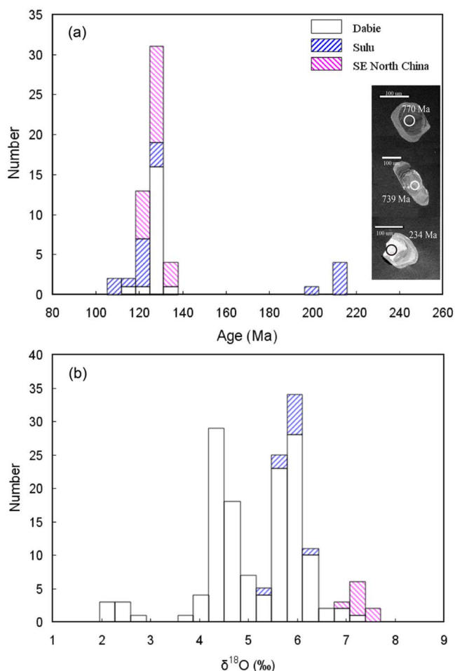
Figure 1 | Histograms of ages (a) and zircon \delta^{18}\text{O} values (b) for Mesozoic mafic igneous rocks in the Dabie-Sulu orogenic belt and its adjacent areas in the southeastern margin of the North China Block. A few zircon cores of Neoproterozoic and Triassic U-Pb ages are present as relicts in voluminous synmagmatic zircon grains of Early Cretaceous U-Pb ages (insert in Fig. 1a).
