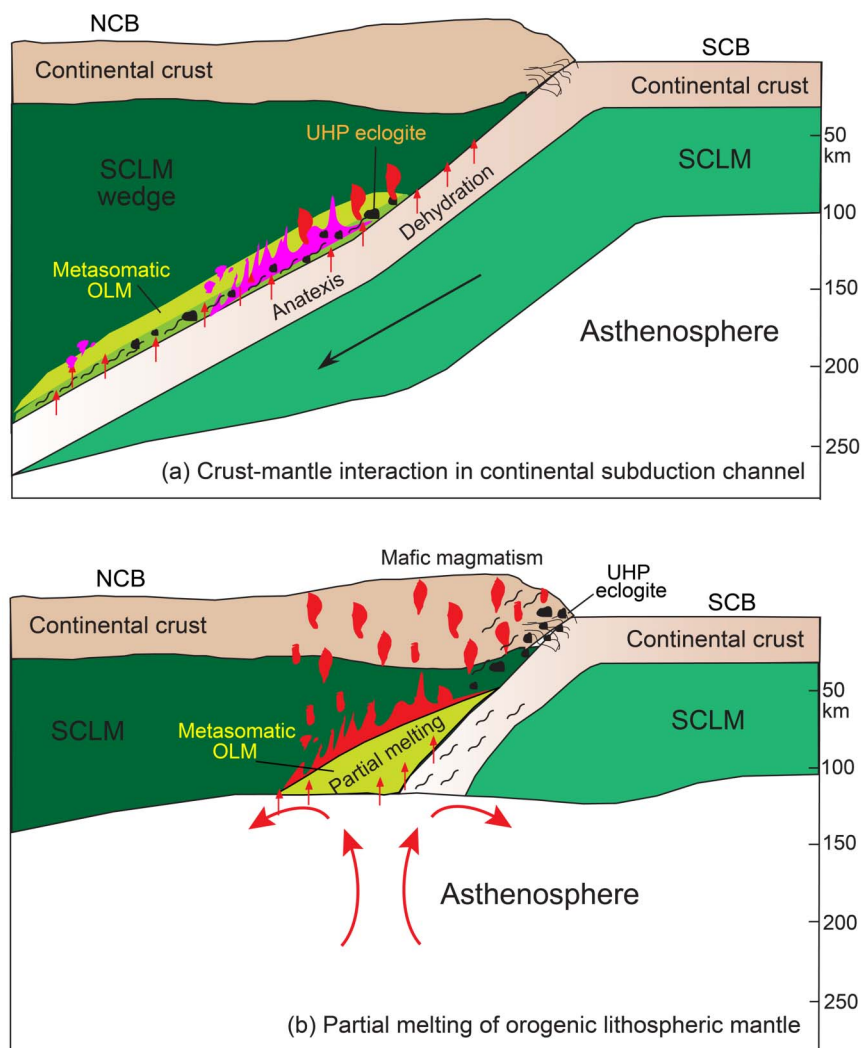
Figure 5 | Schematic cartoon showing crust-mantle interaction and production of postcollisional mafic igneous rocks in continental collision zone. (a) Reaction of the overlying SCLM wedge peridotite with felsic melts derived from the subducted continental crust during the Triassic continental collision in east-central China, generating the metasomes in orogenic lithospheric mantle domains overlying the continental subduction channel. (b) Partial melting of the fertile and enriched SCLM domains in the Early Cretaceous, giving rise to postcollisional mafic igneous rocks. Abbreviations of petrotectonic units: SCB = the South China Block, NCB = the North China Block, UHP = ultrahigh-pressure, SCLM = subcontinental lithospheric mantle, OLM = orogenic lithospheric mantle.
