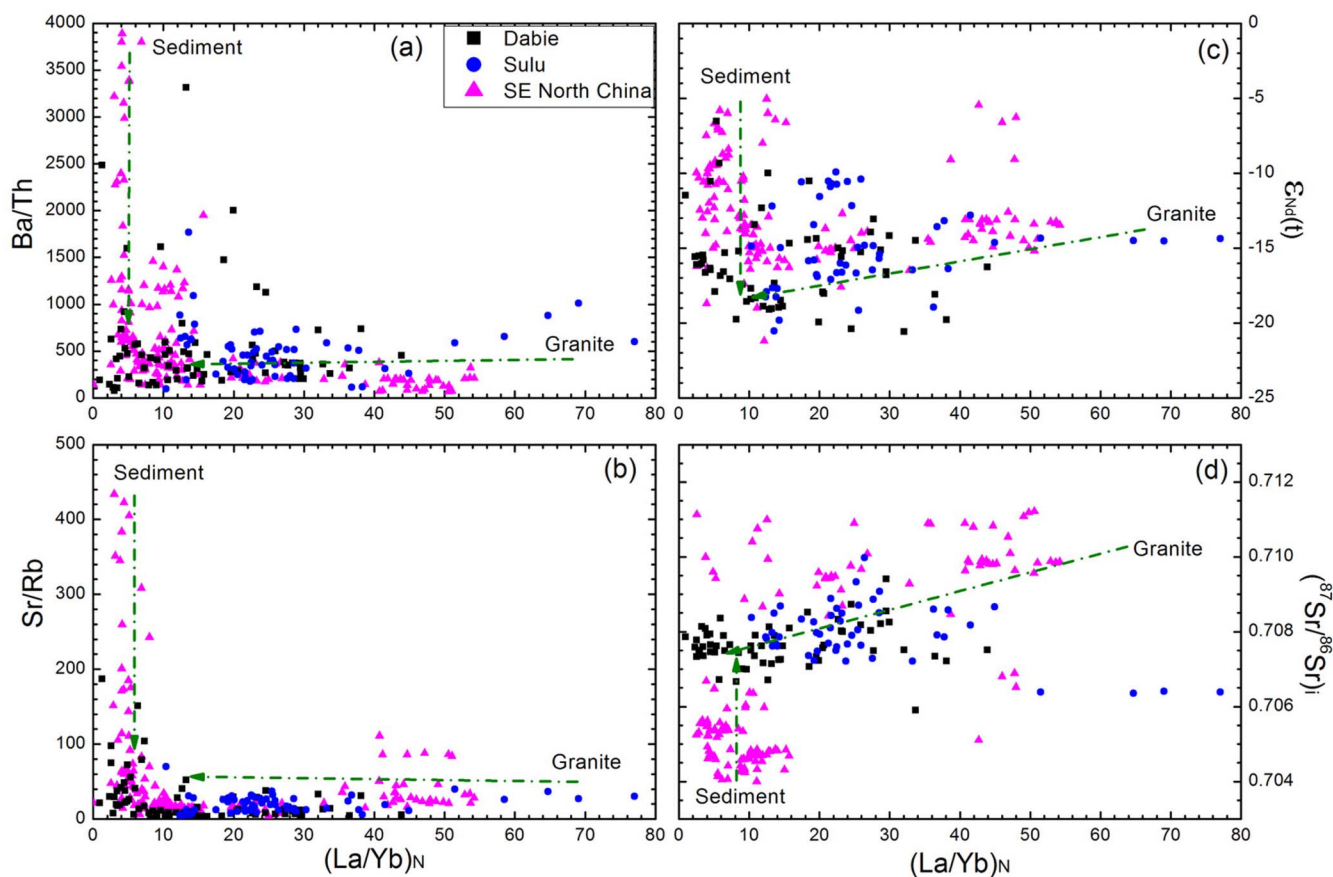
Figure 4 | Plots of whole-rock Ba/Th and Sr/Rb ratios as well as initial Nd-Sr isotope ratios against (La/Yb)_N ratios for postcollisional mafic igneous rocks in east-central China.
