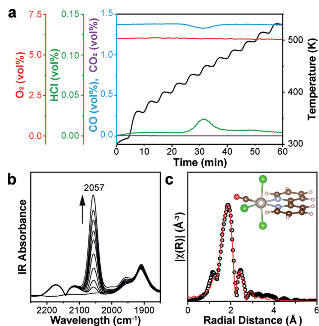
Figure 2. Evolution from [bipy-Ru III Cl 4 ] - to mer (Cl)-[bipy-Ru III (CO)Cl 3 ]. a) Mass spectrometry (MS) showing the outlet gas profile with the corresponding temperature profile under 1%CO and 5%O 2 flow, O 2 is fed to monitor if there is any oxidation of CO to CO 2 . Blue CO, purple CO 2 , red O 2 , green HCl. b) In situ DRIFTS spectra, showing the formation of one terminal CO coordination at 2057 cm -1 . c) Experimental and fitted EXAFS data, suggesting the [bipy-Ru III (CO)Cl 3 ] single-site structures with corresponding DFT calculated models.
