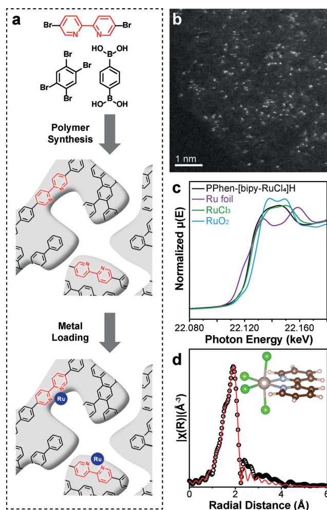
Figure 1. Identification of [bipy-Ru III Cl 4 ] - single site. a) The general approach in creating the single-site coordination environment. b) HAADF-STEM images of PPhen-[bipy-Ru III Cl 4 ]H. c) Ru K-edge XANES spectra of PPhen-[bipy-Ru III Cl 4 ]H, Ru foil, RuCl 3 , and RuO 2 . d) Experimental and fitted EXAFS data of PPhen-[bipy-Ru III Cl 4 ]H. The inlet is the DFT simulation of the [bipy-Ru III Cl 4 ] - structure.
