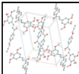
Fig. 2. The molecular packing viewed down the b axis. Dashed lines shows the intermolecular C—H \cdots O hydrogen bonds.
