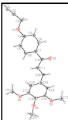
Fig. 1. The structure of showing the atom-numbering scheme and intramolecular hydrogen bond. Displacement ellipsoids are drawn at the 30% probability level.
