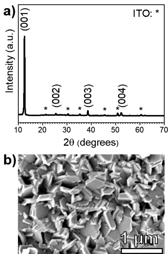
Fig. 3 (a) XRD pattern of a \approx 225 nm thick \text{PbI}_2 film deposited on an SLG/ITO/CdS substrate at T_{\text{source}} = 260^\circ\text{C} , T_{\text{sub}} = 215^\circ\text{C} , P = 1 torr, and t = 20 min. The principal \text{PbI}_2 planes are labeled at their respective diffraction peaks, and the ITO peaks are marked with an asterisk. (b) A plan-view SEM micrograph of the \text{PbI}_2 film.
