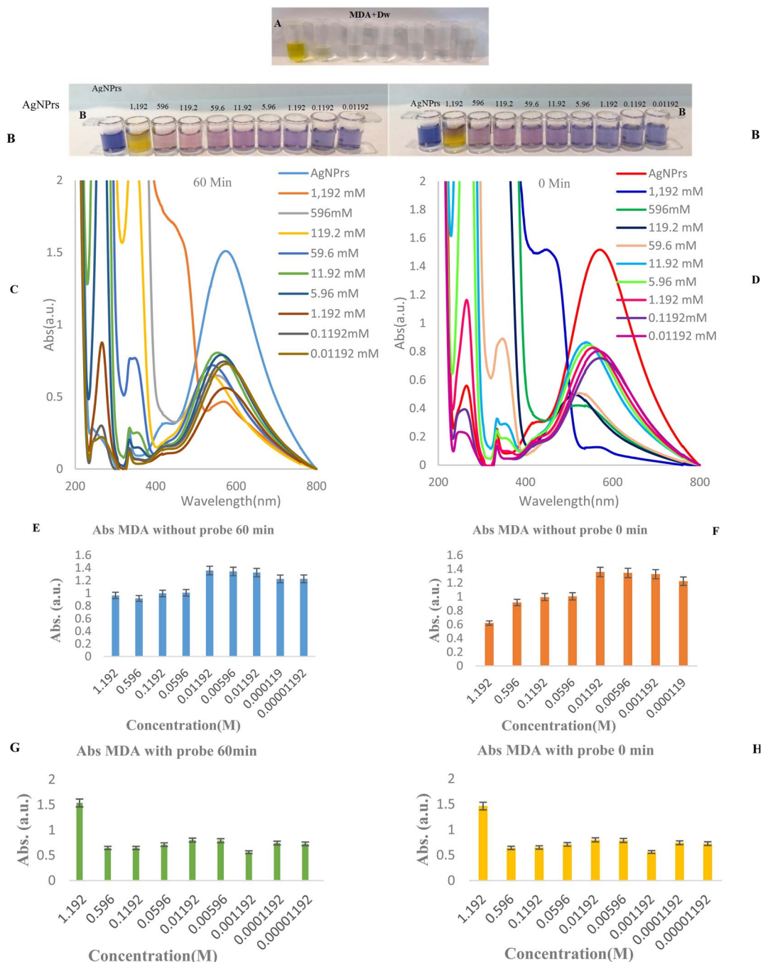
Fig. 2 (A) Digital photos of MDA with deionized water of various concentrations. (B) Colorimetric sensing of AgNPs spiked with various concentrations of MDA at two different incubation times (0 and 60 min), (C) UV-Vis spectra of different concentrations of MDA with AgNPs at a 1 : 1 v/v ratio in 60 min. (D) The UV-Vis spectra of different concentrations of MDA with AgNPs at a 1 : 1 v/v ratio in 0 min. (E) The histogram curve of peak intensity versus MDA concentration without probe from 0.01192 to 1.192 mM after 60 min incubation with a nanoprobe. (F) The histogram curve of peak intensity versus MDA concentration without the probe from 0.01192 to 1.192 mM in the first incubation time [0 min]. (G) A histogram curve of peak intensity versus MDA concentration with the probe from 0.01192 to 1.192 mM at the first incubation time [0 min]. (H) A histogram curve of peak intensity versus MDA concentration with the probe from 0.01192 to 1.192 mM after 60 min incubation with the nanoprobe.
