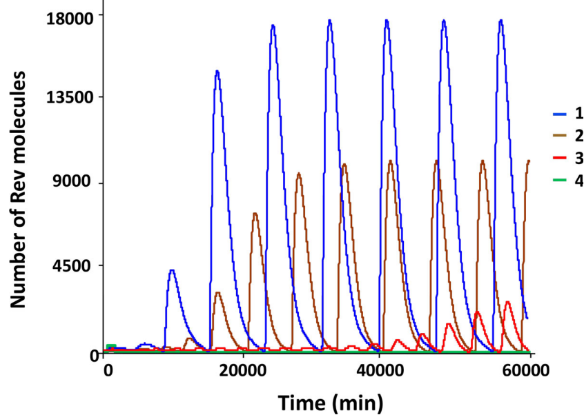
Figure 7 Impact of the Rev mRNA stability on the kinetics of the viral components synthesis in an activated cell. The curves are distinguished by the parameters values: curve 1 - k = 0.0009 \text{ min}^{-1} , curve 2 - k = 0.0014 \text{ min}^{-1} , curve 3 - k = 0.0015 \text{ min}^{-1} , curve 4 - k = 0.0016 \text{ min}^{-1} , k = k_{degr,2kb\_RNA\_Rev\_yyy} , yyy \in \{nuc, cyt\} . Simulations for the version of the model in which the Rev-dependent transport of 9 kb RNA and 4 kb RNA from the nucleus to the cytoplasm leads to the release of the RNA bound Rev proteins into the free cytoplasmic fraction. However, the interaction of Rev with 9 kb- and 4 kb RNAs in the cytoplasm does not take place. The simulations were performed with the model parameter values listed in Table 1.
