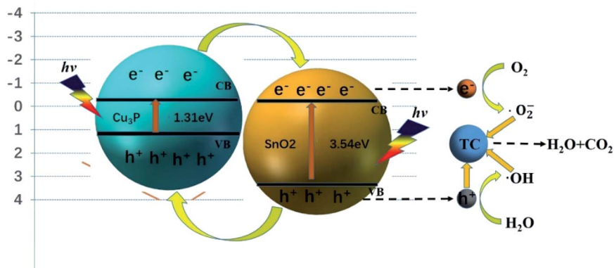
Fig. 8 Mechanism diagram of photocatalytic degradation of TC by heterogeneous \text{Cu}_3\text{P}/\text{SnO}_2 .
