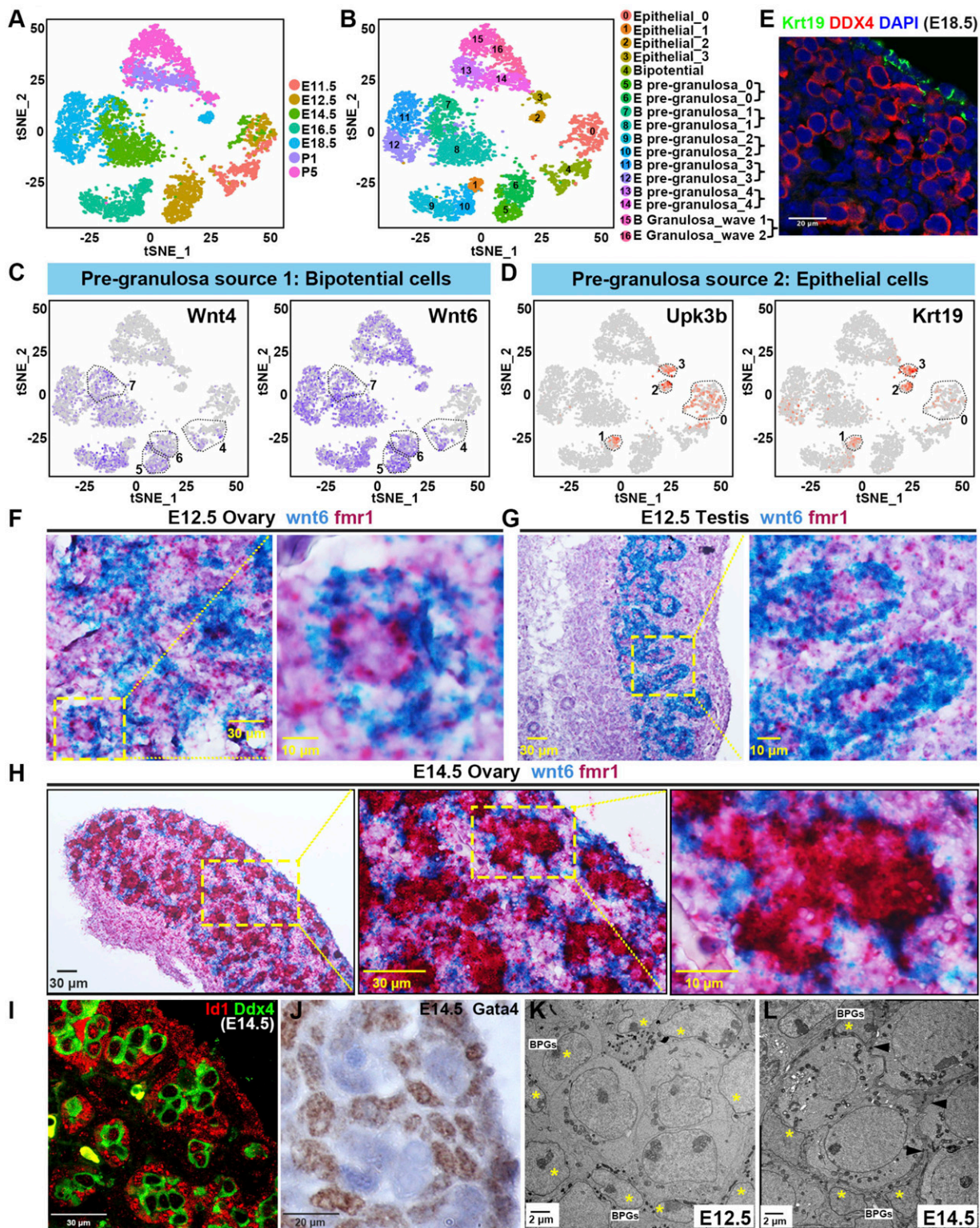
Fig. 3. Identification and cellular localization of epithelial and PG cells. (A) A 2D visualization of clusters from “epithelial” and “pregranulosa” subgroup cells using tSNE. Cells are colored by embryonic time points from E11.5 to P5. (B) A 2D visualization of epithelial and PG cell clusters using tSNE colored by 17 identified cell groups. (C) Expression of Wnt4 and Wnt6 in PG cells; the color indicates level of expression. In C and D, dashed regions correspond to indicated cell clusters (B). (D) Expression of Upk3b and Krt19 of epithelial cells; the color indicates level of expression. (E) Cellular localization of Krt19 in E18.5 ovaries. Ovaries were stained for Krt19, and the germ cell marker DDX4 at E18.5 by immunofluorescence. (F–H) ISH analysis shows Wnt6 (blue) and Fmr1 (red) mRNA expression in the E12.5 ovary (F), E12.5 testis (G), and E14.5 ovary (H). Boxed regions are shown at higher magnification in the Right. (I) Cellular localization of Id1 in E14.5 ovaries. Ovaries were stained for Id1, and the germ cell marker DDX4 at E14.5 by immunofluorescence. (J) Cellular localization of Gata4 in E14.5 ovaries by immunohistochemistry. (K) Electron micrograph of E12.5 ovary showing part of a germline cyst (center) surrounded by BPG cells (yellow asterisks). (L) Electron micrograph of E14.5 ovary showing part of a germline cyst surrounded by BPG cells (yellow asterisks). Squamous membranes of BPG cells surrounding the germ cells are indicated by arrowheads. Scale bars are indicated.
