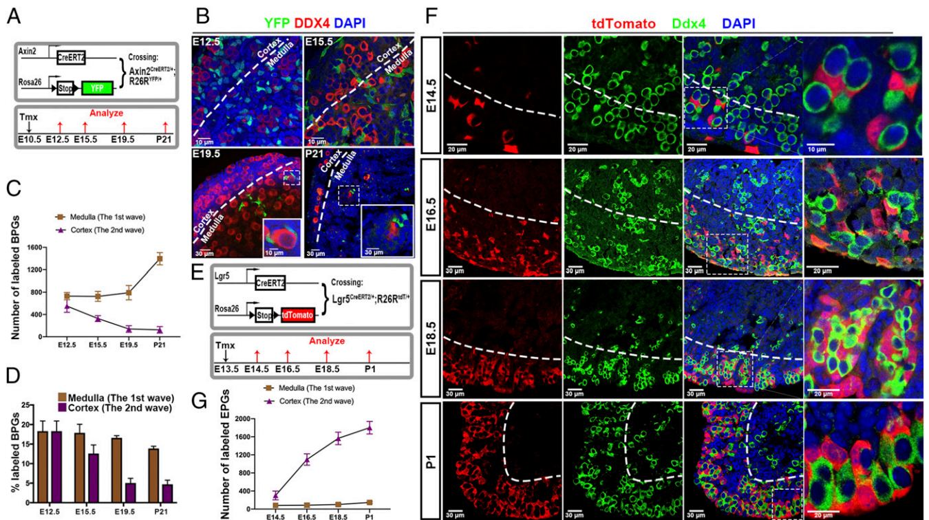
Fig. 5. Lineage tracing of BPG cell replacement by cortical EPG cells. (A) Strategy for lineage-tracing bipotential cells. Mice containing Axin2 CreERT2/+ mice and R26R YFP/YFP received tamoxifen (Tmx) at E10.5, and ovaries were analyzed at E12.5, E15.5, E19.5, and P21. (B) YFP-marked cells (green) are seen adjacent to germ cells (red) in the medulla and in the cortex until E19.5. Boxed regions correspond to Insets . (C) Quantitation of YFP-labeled BPG cells in the cortex and medulla at each time point shown in B. (D) Percentage of cyst/follicle-associated PG cells labeled in the medulla and cortex at each time. (E) Strategy for lineage tracing EPG cells. Mice containing Lgr5 CreERT2/+ and R26R tdT/tdT reporter received Tmx at E13.5, and ovaries were analyzed at E14.5, E16.5, E18.5, and P1. (F) tdTomato-positive EPG cells (red) were sparse at E14.5 but associated with germ cells (green). Cortical tdTomato + cells increased significantly at E16.5, E18.5, and P1, but very few entered the medullar region. Boxed regions correspond to Right Column . (G). Dashed lines in B and F show the boundary of the cortical and medullar regions.
