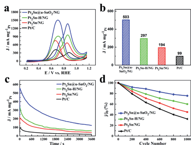
Fig. 5 (a) CV curves of different catalysts in 0.5 M \text{H}_2\text{SO}_4 + 1 M \text{CH}_3\text{OH} solution with a sweep rate of 50 \text{ mV s}^{-1} . (b) The current density of different catalysts at 0.7 V in 0.5 M \text{H}_2\text{SO}_4 + 1 M \text{CH}_3\text{OH} solution. (c) Chronoamperometric curves of different catalysts in \text{N}_2 -saturated 0.5 M \text{H}_2\text{SO}_4 + 1 M \text{CH}_3\text{OH} solution at constant voltage 0.7 V for 3600 s. (d) Changes of peak current densities of the MOR during potential cycling of different catalysts.
