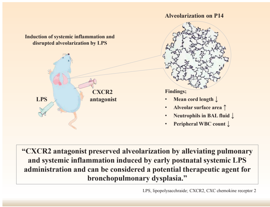
Graphical abstract
