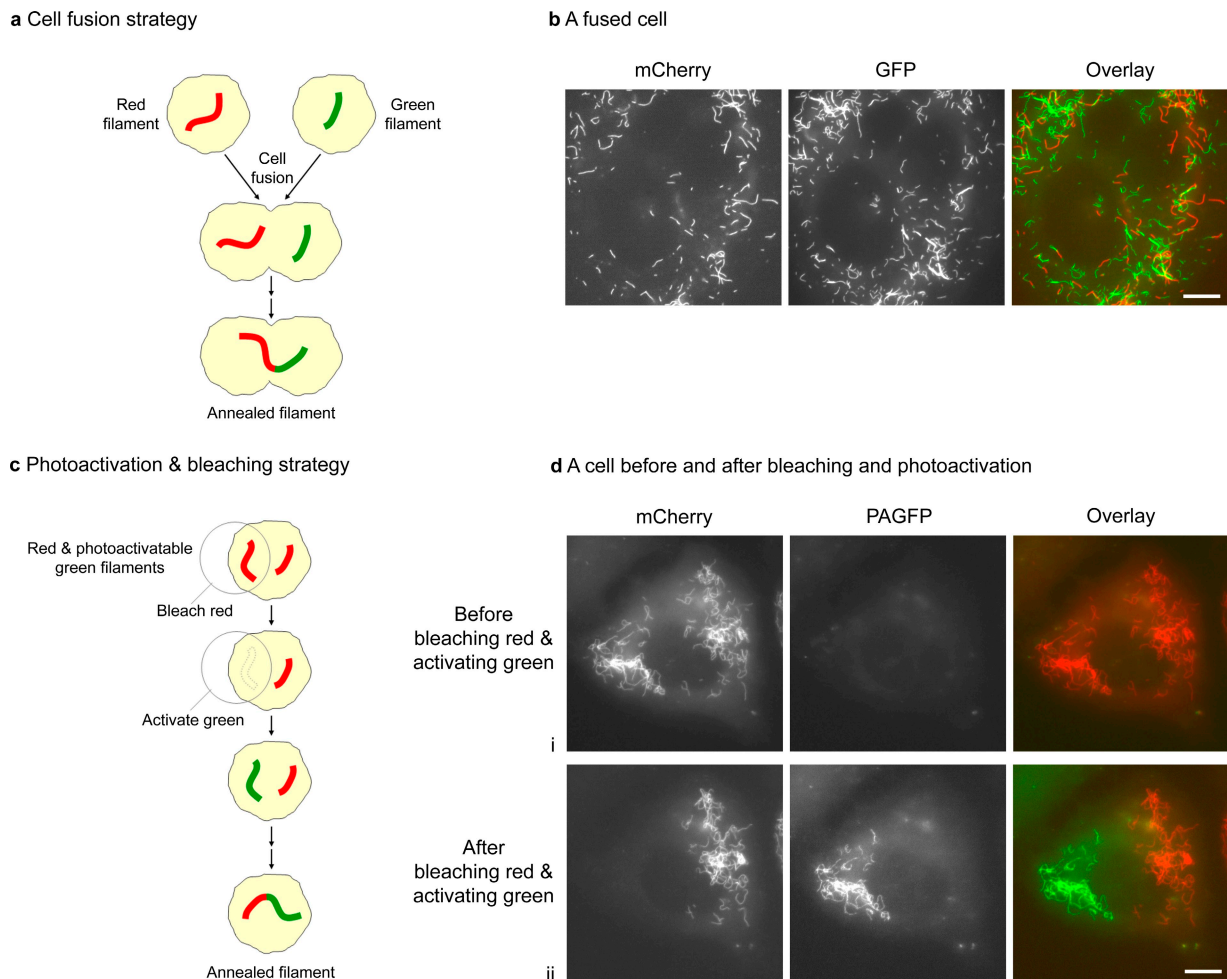
Figure 1. Strategies to test for end-to-end annealing of intermediate filaments. (a) Schematic of the cell fusion strategy. (b) A cell obtained by fusion of SW13 vim - cells coexpressing NFM-mCherry and NFL with SW13 vim - cells coexpressing NFM-GFP and NFL and imaged 3.5 h after fusion. (c) Schematic of the photoactivation and bleaching strategy. (d) An SW13 vim - cell coexpressing mCherry-NFM, PAGFP-NFM, and NFL imaged before bleaching and photoactivation (i), and immediately after bleaching and photoactivation before the filaments had mixed (ii). Bars, 10 \mu m.
