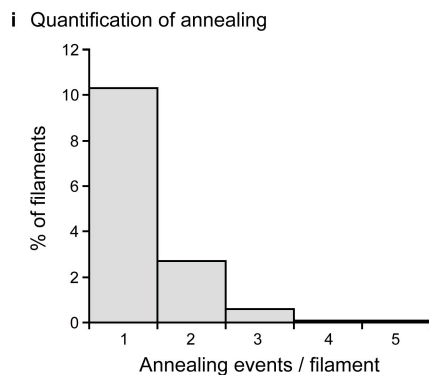
Figure 2. Intermediate filaments undergo end-to-end annealing. Sites of end-to-end annealing (red/green junctions) are marked with white arrowheads. Two examples (i and ii) are shown for each experiment. For clarity, we selected isolated filaments for most of the images. (a) Obtained by fusion of SW13 vim - cells coexpressing mCherry-NFM and NFL with SW13 vim - cells coexpressing GFP-NFM and NFL. (b) Obtained by fusion of SW13 vim - cells coexpressing NFM-mCherry and NFL with SW13 vim - cells coexpressing NFM-GFP and NFL. (c) Obtained by fusion of SW13 vim - cells coexpressing mCherry-vimentin and untagged vimentin with SW13 vim - cells coexpressing GFP-vimentin and untagged vimentin. (d) Obtained by photoactivation and bleaching of SW13 vim - cells coexpressing mCherry-NFM, PAGFP-NFM, and NFL. (e) Excerpts from a video of a neurofilament in a cell formed by the fusion of an SW13 vim - cell coexpressing NFM-GFP and NFL with an SW13 vim - cell coexpressing NFM-mCherry and NFL (Video 1). (f) Obtained by fusion of SW13 vim - cells coexpressing NFM and NFL with SW13 vim - cells coexpressing NFH and NFL. 5 h after fusion, the cells were fixed and immunostained for NFH and NFM. (g) Obtained by fusion of SW13 vim + cells stably expressing mCherry-vimentin with SW13 vim + cells stably expressing GFP-vimentin. (h) The edge of a cell obtained by fusion of SW13 vim + cells stably expressing mCherry-vimentin with SW13 vim + cells stably expressing GFP-vimentin. (i) Frequency distribution of the number of annealing events per filament 2–5 h after fusion of SW13 vim - cells coexpressing NFM-GFP and NFL with SW13 vim - cells coexpressing NFM-mCherry and NFL (991 filaments counted in five cells). NF, neurofilament. Bars, 2 \mu m.
