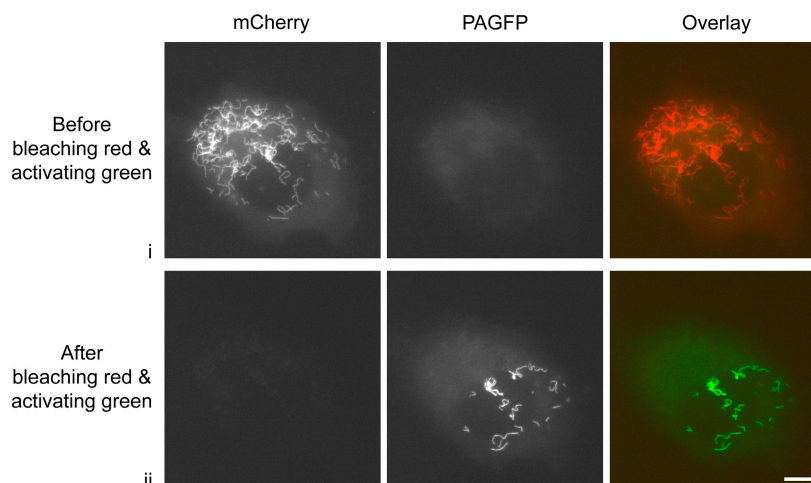
Figure 3. Strategies to test for subunit incorporation along intermediate filaments. (a) Schematic of the cell fusion and photoactivation strategy. (b) A cell obtained by fusion of SW13 vim - cells coexpressing NFL-PAGFP and NFM with SW13 vim - cells coexpressing NFL-mCherry and NFM and imaged before photoactivation (4.5 h after fusion; i) and immediately after photoactivation (ii). (c) Schematic of the photoactivation and bleaching strategy. (d) An SW13 vim - cell coexpressing mCherry-NFM, PAGFP-NFM, and NFL imaged before bleaching and photoactivation (i) and immediately after bleaching and photoactivation (ii). Bars, 10 \mu m.
