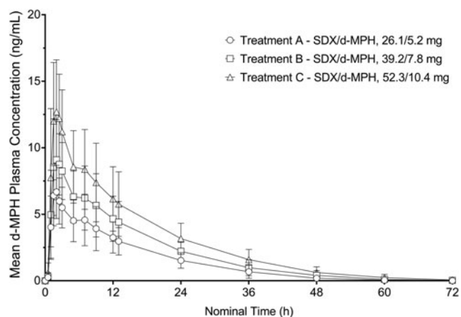
FIG. 1. Plasma concentration–time curve (mean \pm standard deviation) for d-MPH after Treatments A, B, and C. Treatment A: SDX/d-MPH 26.1/5.2 mg; total equivalent d-MPH HCl, 20 mg. Treatment B: SDX/d-MPH 39.2/7.8 mg; total equivalent d-MPH HCl, 30 mg. Treatment C: SDX/d-MPH 52.3/10.4 mg; total equivalent d-MPH HCl, 40 mg. n = 23. d-MPH, dexmethylphenidate; SDX, serdexmethylphenidate.
