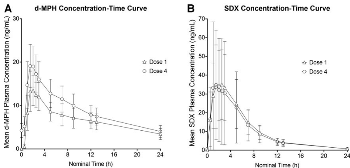
FIG. 3. Plasma concentration–time curve (mean \pm standard deviation) for (A) d-MPH and (B) SDX after 1 and 4 doses of Treatment D: 52.3/10.4 mg SDX/d-MPH, 40 mg total equivalent d-MPH HCl. n=23 . d-MPH, dexmethylphenidate; SDX, serdexmethylphenidate.
