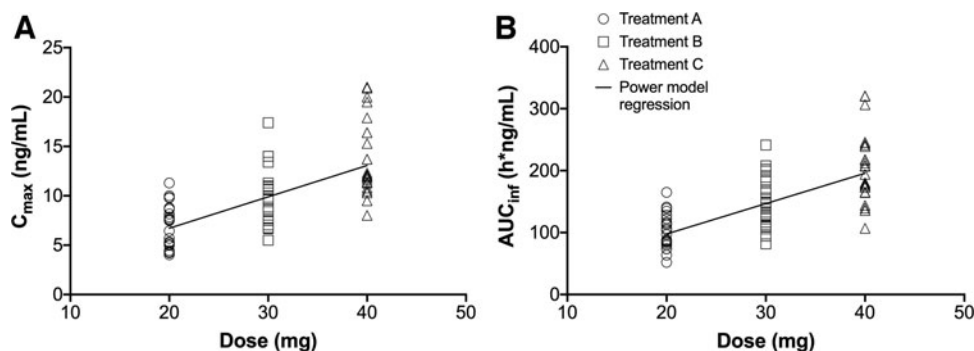
FIG. 2. Power model regression analysis of total equivalent d-MPH dose versus plasma d-MPH (A) C_{max} and (B) AUC_{0-\infty} . (A) Intercept = -0.9812 ; slope = 0.9625 . (B) Intercept = 1.5806 ; slope = 1.0021 . Treatment A: SDX/d-MPH 26.1/5.2 mg; total equivalent d-MPH HCl, 20 mg. Treatment B: SDX/d-MPH 39.2/7.8 mg; total equivalent d-MPH HCl, 30 mg. Treatment C: SDX/d-MPH 52.3/10.4 mg; total equivalent d-MPH HCl, 40 mg. n=23 . AUC_{0-\infty} , area under the concentration–time curve from time-zero extrapolated to infinity; C_{max} , maximum concentration in plasma; d-MPH, dexmethylphenidate; SDX, serdexmethylphenidate.
