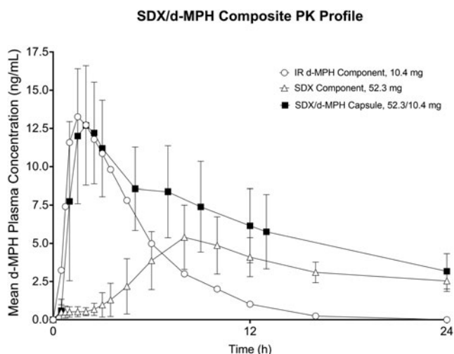
FIG. 4. Plasma concentration–time curve (mean ± standard deviation) for immediate-release d-MPH 10.4 mg, SDX 52.3 mg, and SDX/d-MPH 52.3/10.4 mg. The profile for IR d-MPH is included for comparison and was inferred from data reported in the summary basis of approval for d-MPH (Focalin®). Available from https://www.accessdata.fda.gov/drugsatfda_docs/nda/2001/21-278_Focalin_medr_P1.pdf . IR, immediate-release; MPH, methylphenidate; SDX, serdexmethylphenidate.
