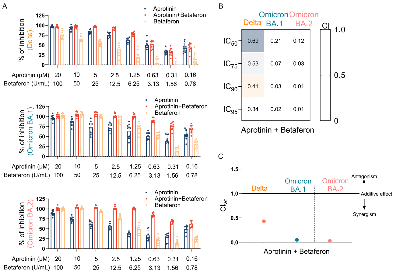
Fig. 2. Antiviral effects of aprotinin in combination with interferon-β (betaferon) against Delta, Omicron BA.1, and Omicron BA.2 isolates. Betaferon was tested in a fixed combination with aprotinin in SARS-CoV-2 (MOI 0.01)-infected Caco-2-F03 cells. Values represent mean ± S.D. of three independent experiments. B) Combination indices were calculated at the IC 50 , IC 75 , IC 90 , and IC 95 levels following the method of Chou and Talalay. C) The weighted average CI value (CI wt ) was calculated according to the formula: CI wt [CI 50 + 2CI 75 + 3CI 90 + 4CI 95 ]/10. A CI wt <1 indicates synergism, a CI wt =1 indicates additive effects, and a CI wt >1 suggest antagonism.
