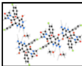
Fig. 2. A partial packing diagram for the title compound. Hydrogen bonds are shown as dashed lines.
