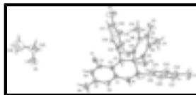
Fig. 1. The molecular structure of the title molecule, with the atom-numbering scheme. Displacement ellipsoids are drawn at 30% probability level.
