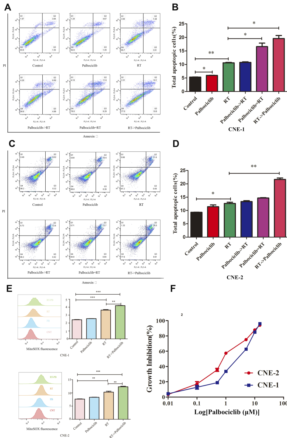
Figure 3 Palbociclib induced apoptosis in irradiated CNE-1 and CNE-2 cells. Cells were treated with IC50 concentration of palbociclib for 48 hrs, radiation, palbociclib before, after or concurrent with radiation at a dose of 6 Gy, and then detected by flow cytometry after staining with Annexin V-FITC/PI. (A) The apoptosis rate of CNE-1 cells receiving palbociclib concurrently (Palbociclib=RT) and after radiation (RT->Palbociclib) was significantly higher. (C) CNE-2 cells exposed to palbociclib following RT markedly prompted apoptosis. (B, D) Histogram represented the total apoptotic rate (late + early phase) of CNE-1 and CNE-2 cells. (E) Palbociclib increased mitochondrial ROS levels in irradiated CNE-1 and CNE-2 cells. Cells were treated with palbociclib, radiation and combined regimen (RT->Palbociclib), and they were detected by flow cytometry. CNE-1 and CNE-2 cells exposed to radiation at a dose of 6 Gy significantly elevated mitochondrial ROS levels and palbociclib further elevated mitochondrial ROS levels in irradiated cells. (F) CNE-1 and CNE-2 cells were incubated with increasing concentrations of palbociclib for 72 hrs. Cell viability was determined with CCK8 assay (n=3 per group). All data represented as mean ± s.d. from three independent experiments. * P < 0.05; **P < 0.01; ***P < 0.001.
