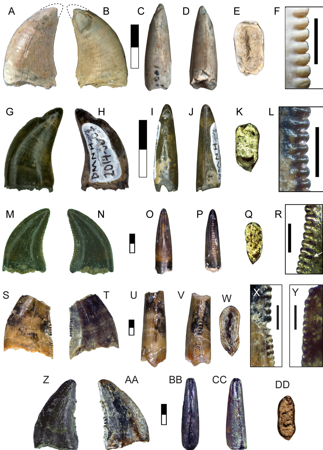
Figure 6 Teeth assigned to Dromaeosauridae . DMNH 2013-07-1080 shown in lingual (A), labial (B), mesial (C), distal (D) and basal views (E); lateral view of distal denticles (F). DMNH 2014-06-02 shown in lingual (G), labial, (H), mesial (I), distal (J), and basal (K) views; lateral view of distal denticles (L). SMU 73779 shown in lingual (M), labial (N), mesial (O), distal (P) and basal views (Q); lateral view of distal denticles (R). SMU 77217 shown in labial (S), lingual (T), mesial (U), distal (V), and basal (W) views; Z, AA, BB, CC, DD.
