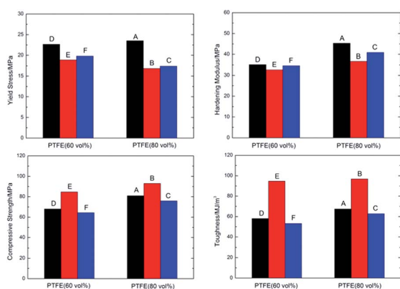
Fig. 4 Comparison of mechanical properties parameters of six types of fluorine-containing thermite.
