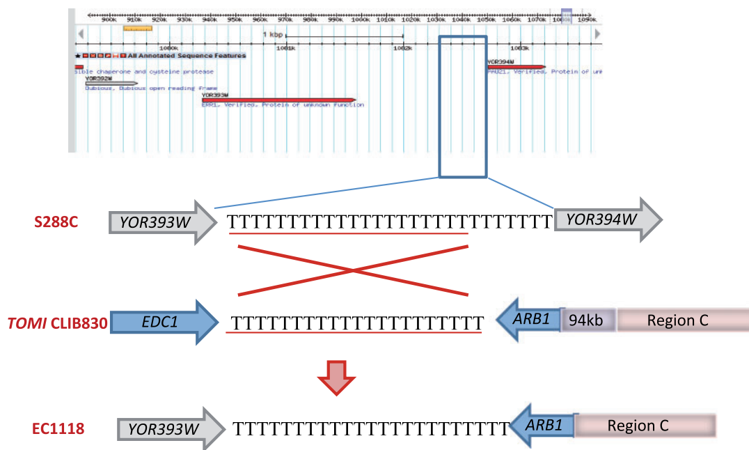
Fig. 4. Mechanism of insertion of region C by homologous recombination between poly(T) sequences located upstream of the region C in Torulaspota microellipsoides and downstream of YOR393W on Saccharomyces cerevisiae chromosome XV.
