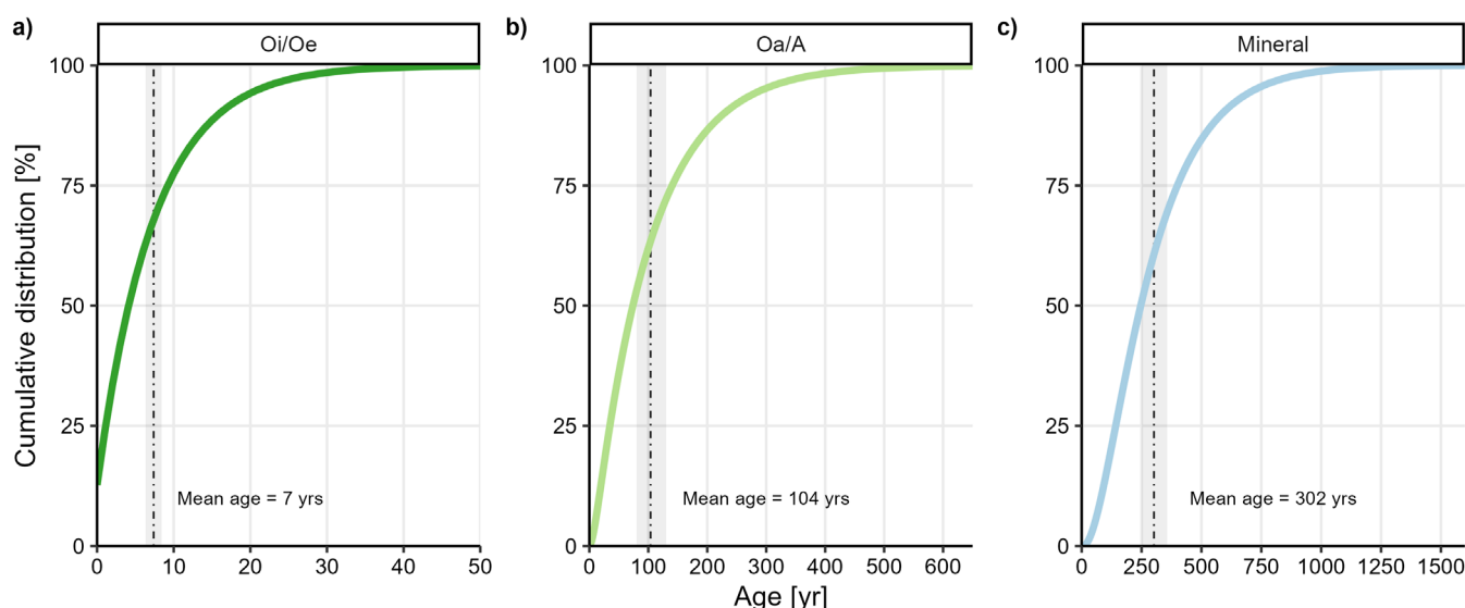
FIGURE 3 | Cumulative soil organic carbon (SOC) pool ages for all three layers/pools: (a) Oi/Oe, (b) Oa/A, and (c) mineral (0–10 cm) based on the three-pool model using the full dataset (1969–2023). Mean SOC ages (black dashed lines) and 95% credible intervals (shaded grey areas) are derived from a subset of accepted model parameters from the Bayesian Markov chain Monte Carlo procedure to calculate the probability distribution of SOC ages for each pool (see 2. Methods).
