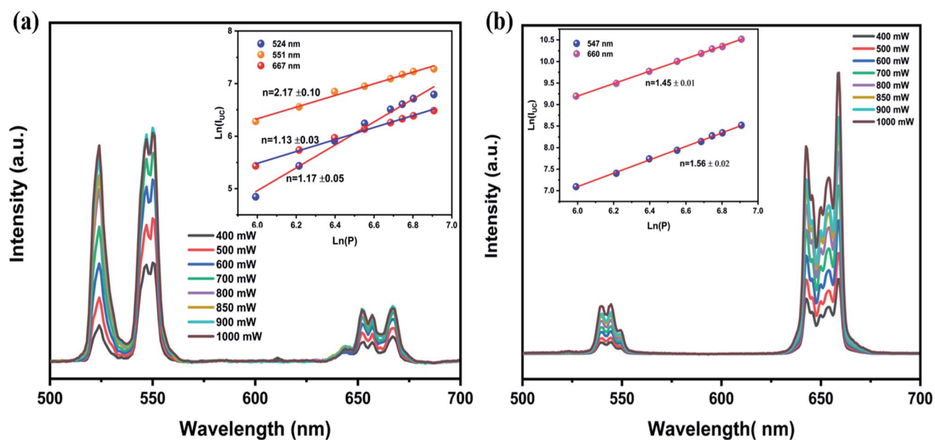
Fig. 7 Represents the variation UC emission at different pump powers, inset shows the dependences of \ln(I_{UC}) on \ln(P) : (a) for \text{LiZnPO}_4:\text{Er}^{3+}/\text{Yb}^{3+} . (b) For \text{LiZnPO}_4:\text{Ho}^{3+}/\text{Yb}^{3+} .
