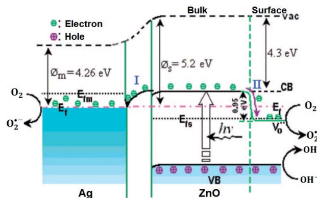
Fig. 3 Photogenerated electron transfer in Ag/ZnO nanocatalyst during the catalytic process. E_F : Fermi level; V_O^{\bullet\bullet} : oxygen vacancy; VB: valence band; CB: conduction band; m: metal; vac: vacuum level; and s: semiconductor. 52
