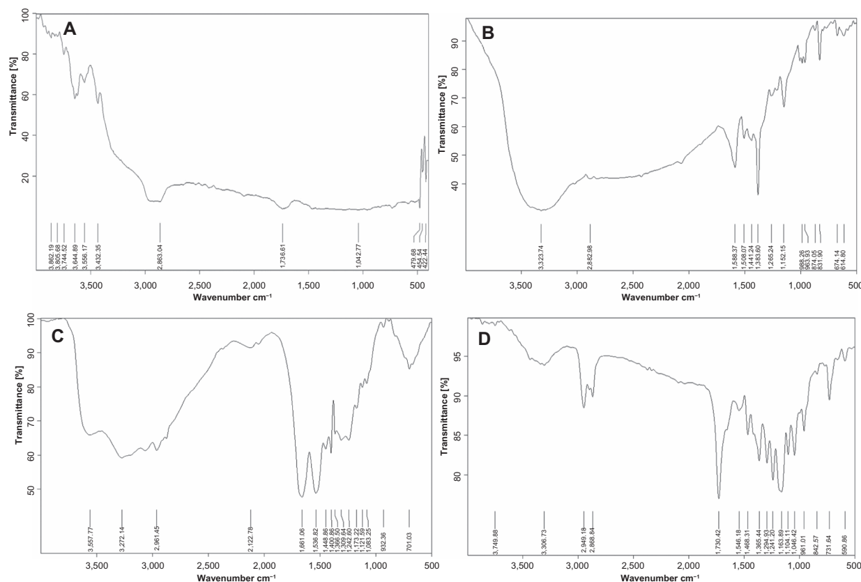
Figure 2 Fourier transform infrared spectra. (A) PCL spectra showing transmittance peaks for standard PCL. (B) Standard resveratrol spectra showing a typical trans olefinic band at 930–961 \text{cm}^{-1} . (C) RNP spectra depicting albumin and characteristic resveratrol bands. (D) Standard PCL-RNP spectra show bands characteristic for PCL (2,900–2,800 \text{cm}^{-1} ), resveratrol (930–961 \text{cm}^{-1} ), and albumin.
