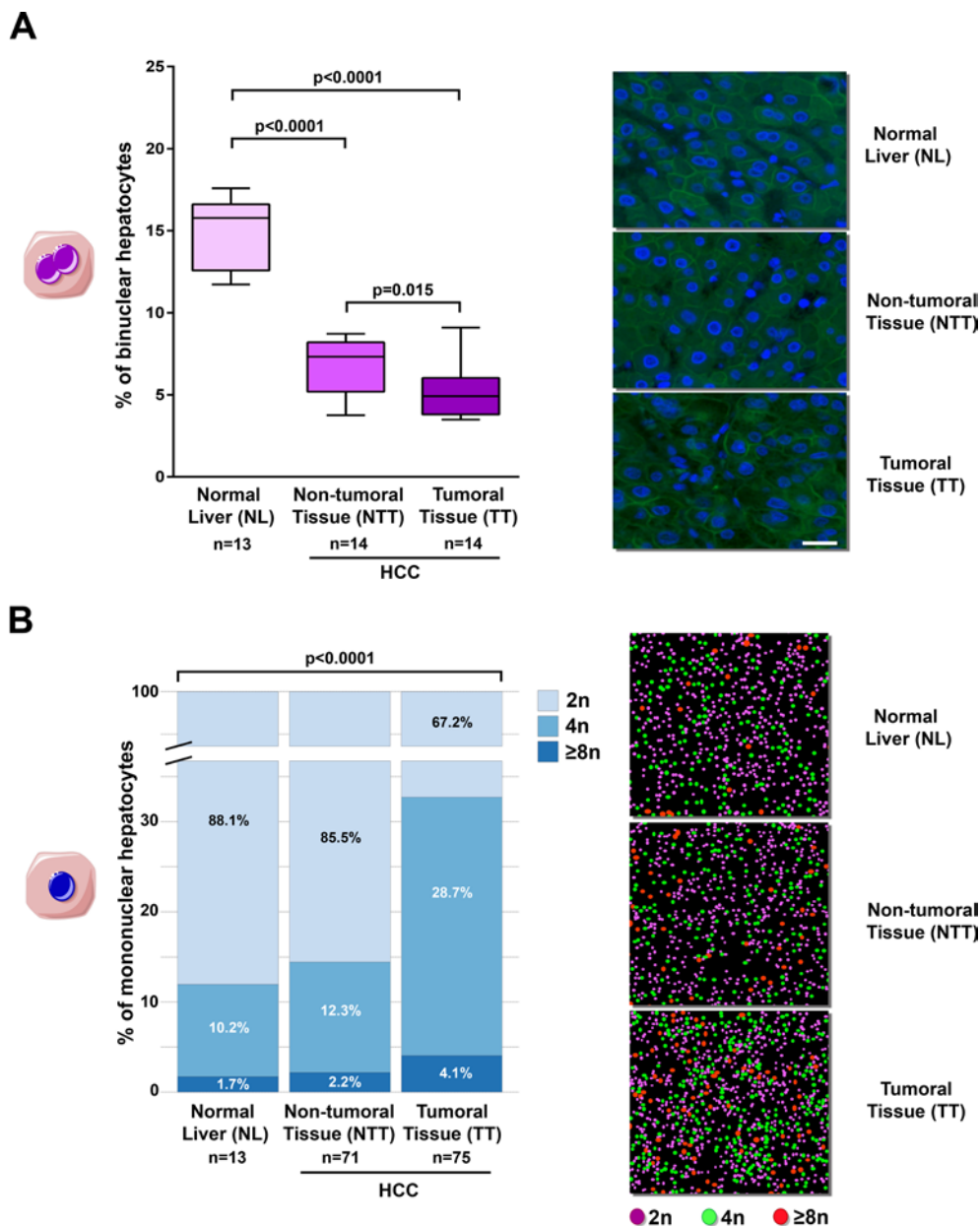
Figure 2 Cellular and nuclear ploidy spectra during human liver carcinogenesis. (A) Left panel: box plots for the percentage of binuclear hepatocytes ( 2 \times 2n and 2 \times \geq 4n ) relative to total hepatocytes population. The bottom, central and top lines of each box represent the first quartile, median and third quartile of the distribution, respectively ( n=13 for normal liver [NL], n=14 for non-tumorous tissue [NTT] and HCC tumorous tissue [TT]). Values represent the mean \pm SEM. Data were compared using Kruskal-Wallis test. Right panel: representative magnification images (scale bar: 40 \mu\text{m} ) highlight binuclear and mononuclear hepatocytes in NL, NTT and HCC TT. (B) Left panel: percentage of mononuclear 2n , 4n and \geq 8n hepatocytes relative to total mononuclear hepatocytes in each group (NL, NTT and TT); n corresponds to the number of patients analysed. Data were compared using multivariate analysis of variance (MANOVA). Right panel: representative higher magnification images of nuclear ploidy spectrum (NL, NTT, TT). HCC, hepatocellular carcinoma.
