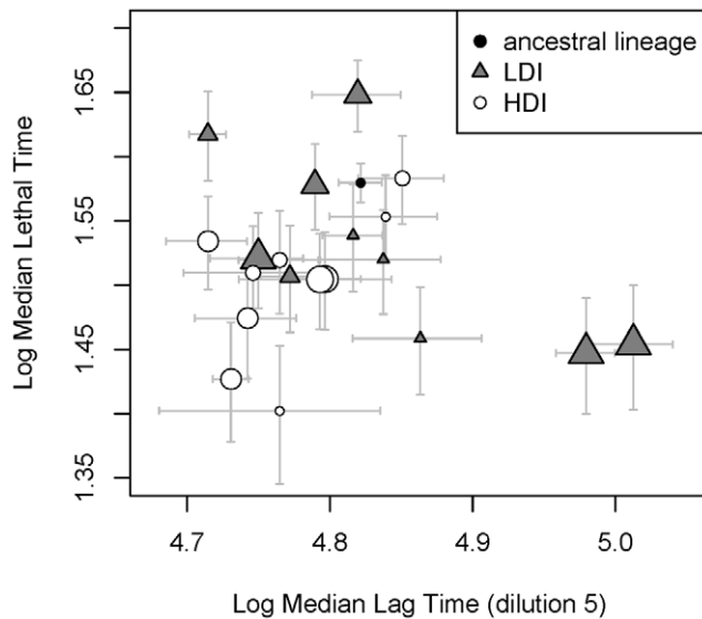
Figure 5. Median lethal time (i.e. the time at which 50% of the insects injected with a particular lineage are dead) as a function of median lag time (i.e. the time at which 50% of the populations of a particular lineage have overreached the absorbance of an empty well). The estimation of these times are performed using a parametric survival regression method (see method). Horizontal and vertical bars correspond to the standard error of these estimates. In LDI lineages, the two quantities are negatively correlated, indicating that the fastest growing LDI lineages are the least virulent. No relation could be found between median lag time and median lethal time in HDI lineages. The size of symbols indicates the proportion of clones that display the total haemolysis phenotype. When analyzing both ancestral and selected lineages, we found a marginally significant link between this variable and virulence. doi:10.1371/journal.pone.0015872.g005
