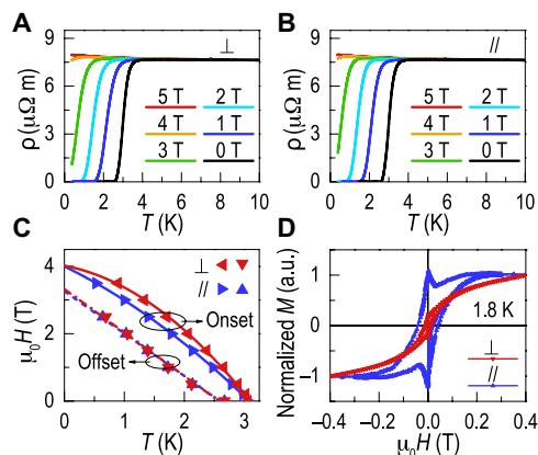
Fig. 1. Coexistent superconductivity and ferromagnetism in hydrogenated boron-doped diamond. Resistive superconducting transitions in (A) perpendicular ( \perp ) and (B) parallel ( // ) applied magnetic fields, respectively. (C) The temperature dependences of the critical field, \mu_0 H(T) , measured in magnetic fields perpendicular and parallel to the sample. To build up the \mu_0 H - T phase boundaries, a criterion was set at 95% of the normal-state resistivity to determine the onset critical temperature, and the resistive superconducting transition was linearly extrapolated down to \rho = 0 for the determination of the offset critical temperature in different magnetic fields. The \mu_0 H - T phase boundaries are extrapolated to zero temperature by quadratic fits (solid curves) and linear fits (dashed lines), respectively. (D) Magnetization hysteresis loops measured at 1.8 K in magnetic fields perpendicular and parallel to the sample. The magnetization, M , is normalized to its value at 0.4 T. a.u., arbitrary units.
