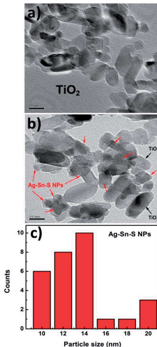
Fig. 2 TEM images of (a) 30 nm bare TiO 2 nanoparticles, (b) Ag 8 SnS 6 nanocrystals deposited on TiO 2 nanoparticles and (c) size distribution of Ag 8 SnS 6 nanocrystals.
