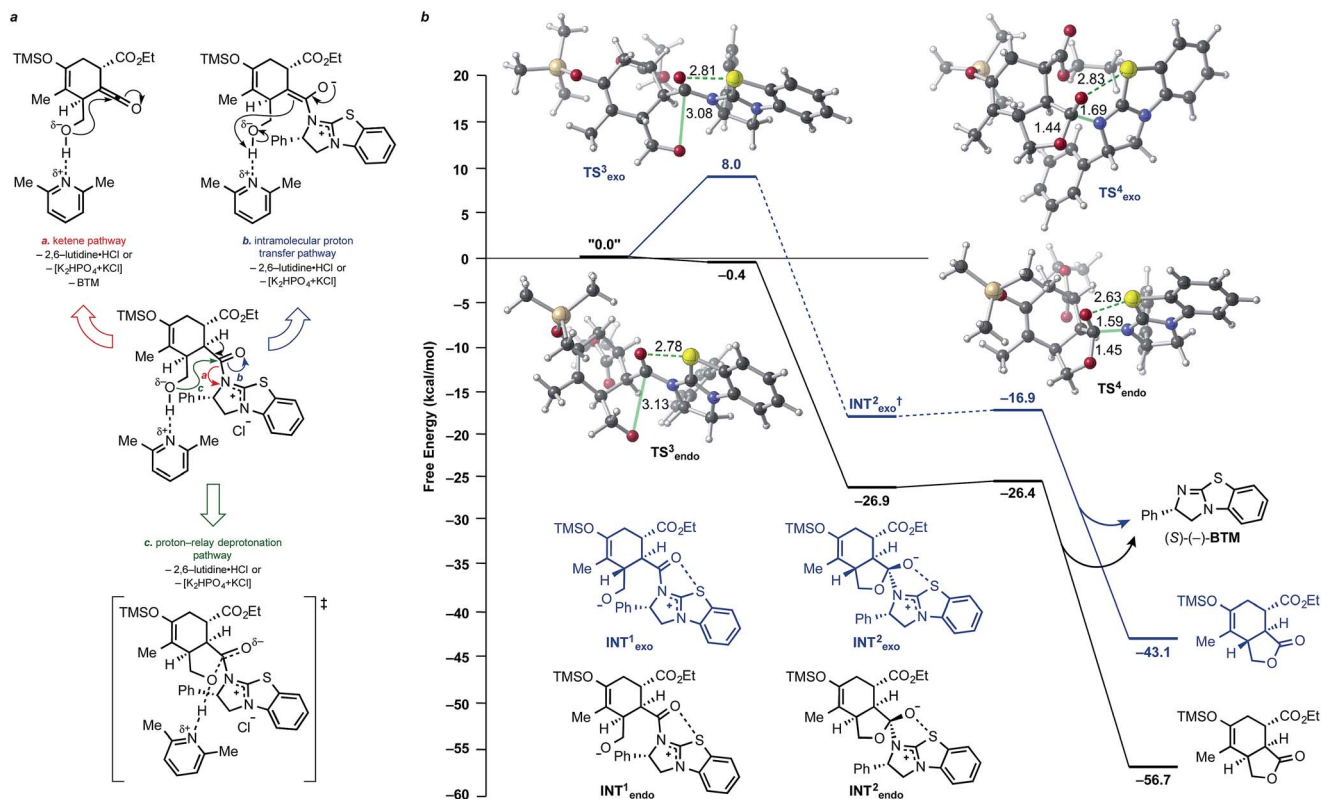
Fig. 9 (a) Possible lactonization pathways for the DAL organocascade process. (b) Computed potential energy surface for the lactonization step of the DAL. Free energies (kcal mol -1 ) were calculated employing SMD(DCM)-M06-2X/6-31G(d). Intermediates and optimized TSSs for both endo (black) and exo (blue) pathways are shown. Selected bond distances are shown (Å).
