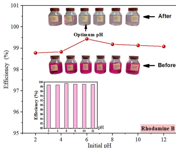
Fig. 6 Rhodamine B removal efficiencies as a function of initial pH of treated solutions ( [Rhodamine\ B]_0 = 10\text{ mg L}^{-1} ; pH = 2 to 12; OSB = 4 g L -1 ; contact time = 1 h; T = 20\text{ }^\circ\text{C} ).
