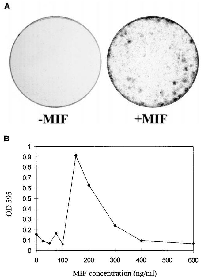
Figure 4. (A) Primary MEFs show extended life span in the presence of 200 ng/ml rMIF. Cells one passage before senescence were plated in the presence and absence of MIF, and stained after 15 d. Numerous colonies were formed only in the presence of MIF. (B) Dose dependency of MIF treatment in inducing extended life span. Primary cells, as in A, were grown in the presence of varying concentrations of MIF. After 17 d, cells were crystal violet stained, and washed. Resolubilized crystal violet was assayed as a measure of cell density.
