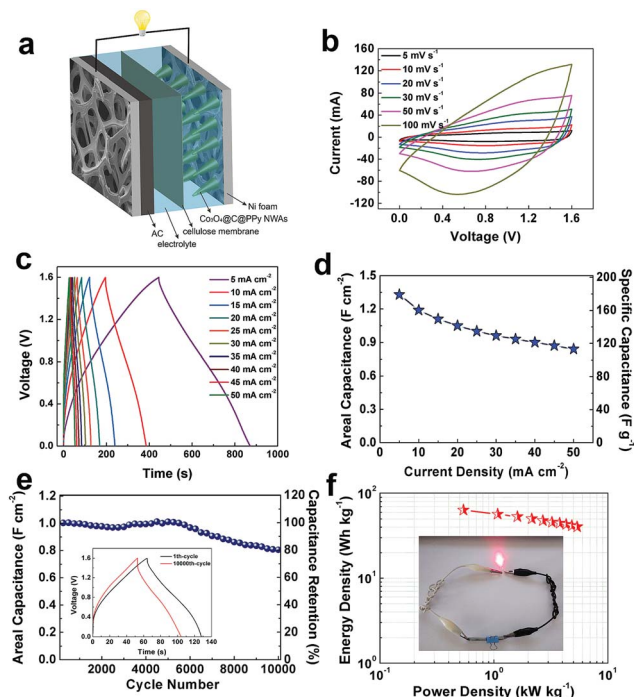
Fig. 8 The electrochemical performances of \text{Co}_3\text{O}_4\text{@C@PPy//AC} device. (a) Schematic illustration of the assembled ASC; (b) CV profiles collected at various scan rates; (c) galvanostatic charge–discharge curves collected at various current densities; (d) areal capacitance and specific capacitance of the ASC at different current densities; (e) capacitance retention of the ASC in 10 000 galvanostatic charge–discharge cycles at 25 \text{ mA cm}^{-2} , inset: profiles of the first and the 10,000th charge–discharge cycle; (f) Ragone plots of the \text{Co}_3\text{O}_4\text{@C@PPy//AC} ASC device, inset show the photograph of the red LED powered by the device.
