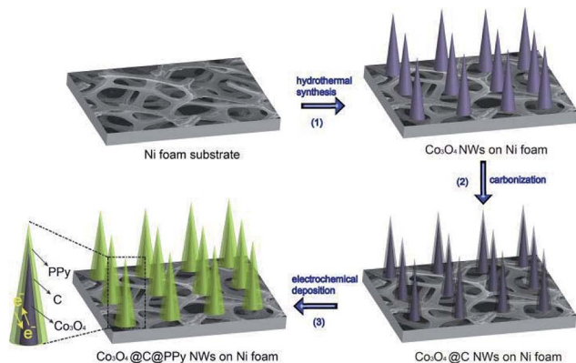
Fig. 1 Schematic of fabrication of sandwich structural \text{Co}_3\text{O}_4@\text{C}@PPy .
