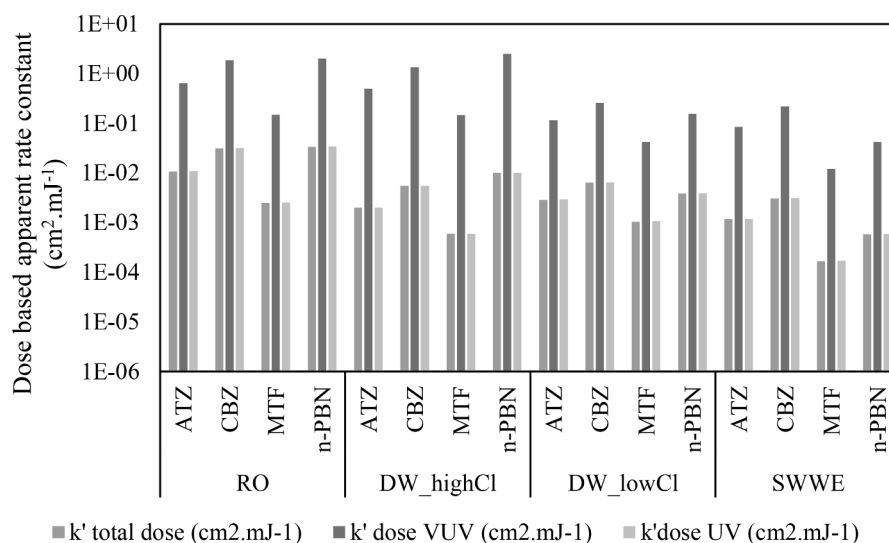
Fig. 3. Comparison of k'_{totaldosed} , k'_{UVdosed} and k'_{VUVdosed} of atrazine (ATZ), carbamazepine (CBZ), metformin (MTF) and n-butyl paraben (n-PBN) in various water types using VUV+UV AOP. Experiments were performed in a 2 cm pathlength cell for DW_highCl sample and the rest in 1 cm pathlength cell.
