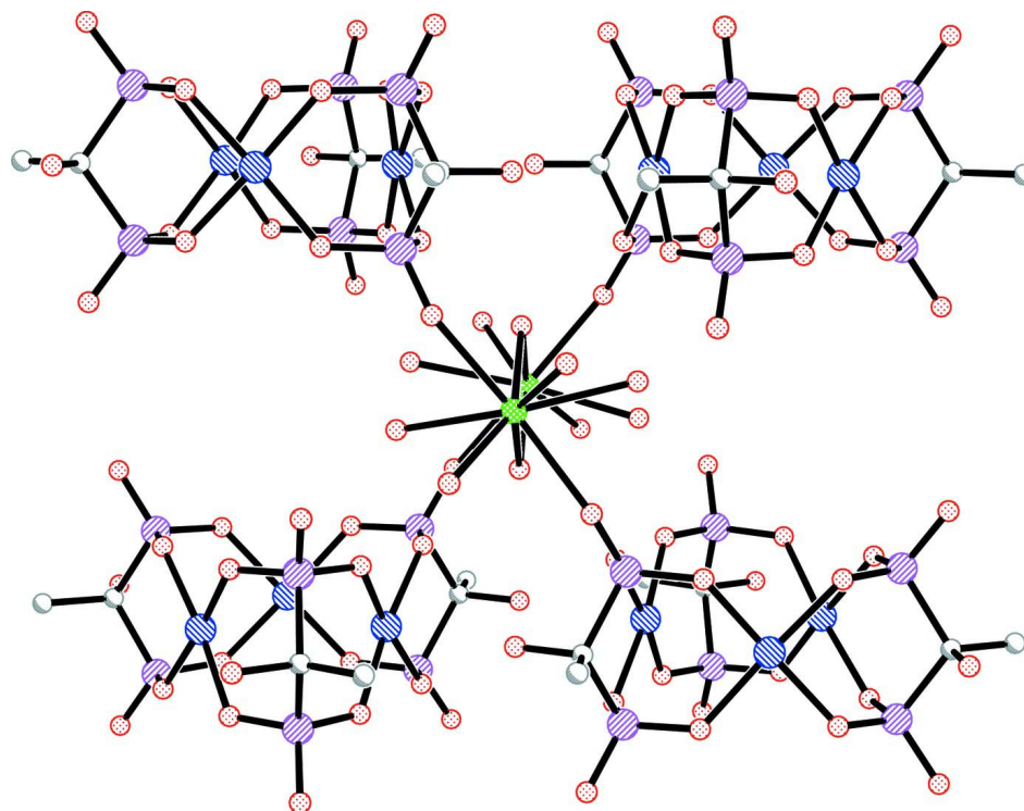
Figure 3 Linking of cations to anions of adjacent layers in crystal packing.
