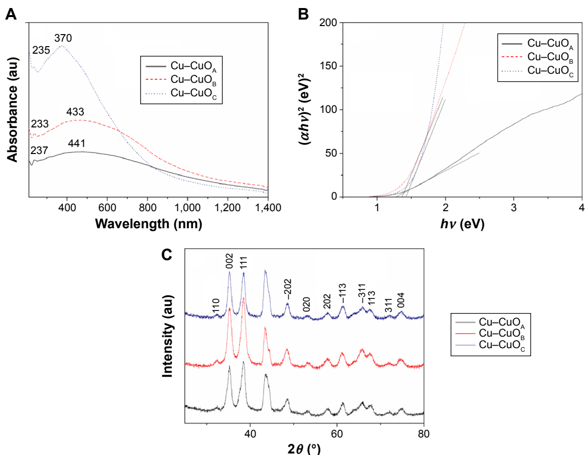
Figure 4 Optical and structural characteristics of Cu–CuO. Notes: (A) UV-vis spectra. (B) Plot of (\alpha hv)^2 vs h\nu . (C) XRD diffractogram of Cu–CuO. Abbreviations: UV-vis, ultraviolet-visible; XRD, X-ray diffractogram.
