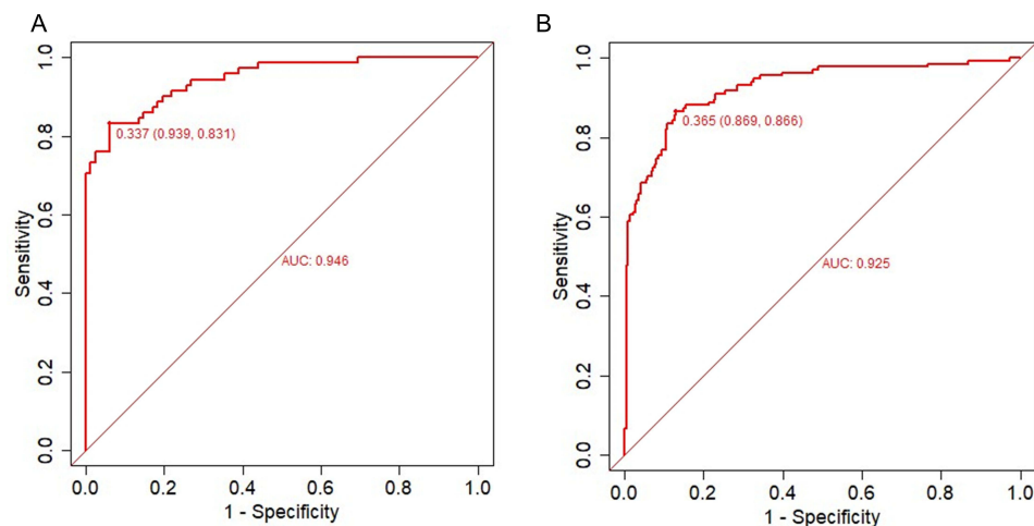
Figure 5 Receiver operating (ROC) curves of nomogram based on the data of the (A) training set and (B) validation set.
