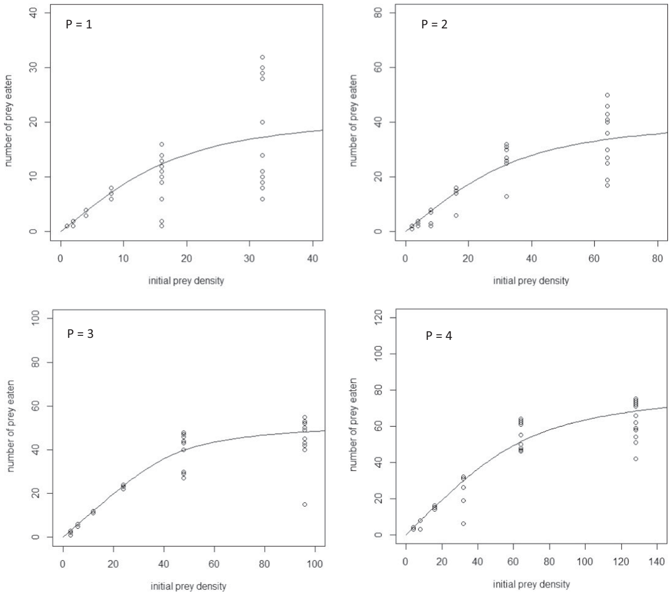
FIGURE 2 Fitting of the Crowley–Martin model to Macrolophus pygmaeus 5th-instar nymph functional response data. P denotes the predator density
