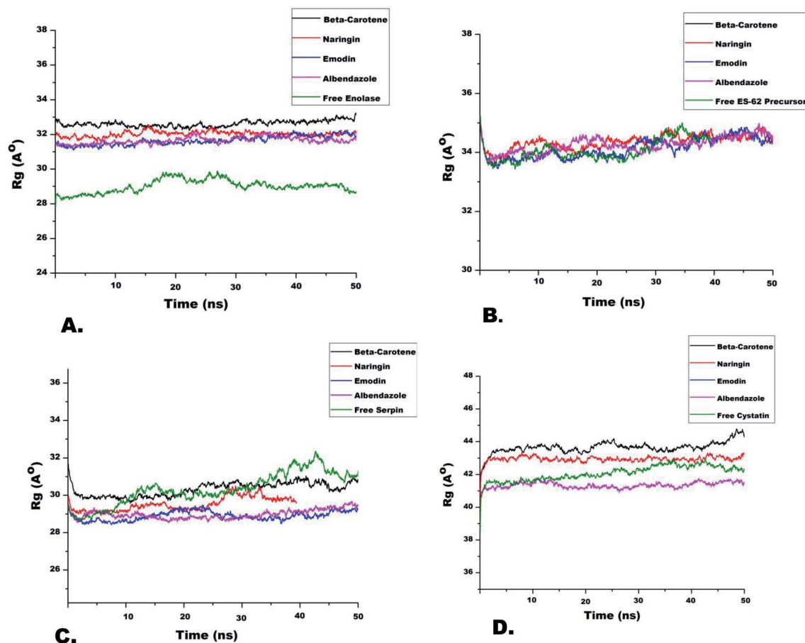
Fig. 4 R_g analysis of filarial immune-modulatory proteins with anti-filarial drug and nutraceutical compound complexes in molecular dynamics simulation for the time scale of 50 ns: (A) enolase, (B) ES-62 precursor, (C) serpin and (D) cystatin.
