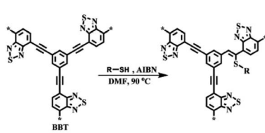
Fig. 7 Synthesis of functionalized BBT via thiol–yne click reaction and its possible structures. Adapted with permission. 119 Copyright 2019, Royal Society of Chemistry.
