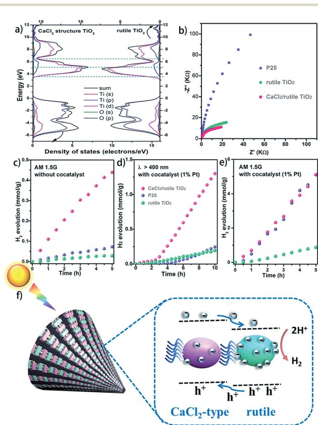
Fig. 6 Photocatalytic performance of \text{CaCl}_2/\text{rutile TiO}_2 . (a) Calculated density of states (DOS) of \text{CaCl}_2 structured \text{TiO}_2 and rutile \text{TiO}_2 ; (b) Nyquist plots of the EIS for \text{CaCl}_2 structured \text{TiO}_2 , P25, and commercial rutile \text{TiO}_2 (Ref.rutile); Water splitting hydrogen evolution activities for \text{CaCl}_2/\text{rutile TiO}_2 , commercial rutile \text{TiO}_2 (Ref.rutile), and P25: (c) without any cocatalyst under simulated sunlight (with an AM 1.5G filter), (d) with the assistance of 1% Pt as the cocatalyst under simulated sunlight (with an AM 1.5G filter) and (e) visible light (wavelength > 400 nm) illumination. (f) Schematic diagram for the electron transfer process under the illumination of light for \text{CaCl}_2/\text{rutile TiO}_2 .
