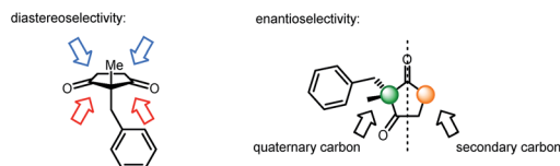
Fig. 2 Origin of stereoselectivities in mono-reduction of 1,3-diketones.
