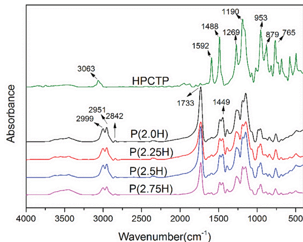
Fig. 2 FTIR spectra of HPCTP and P(H) microcapsules.
