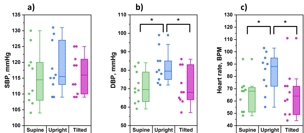
Figure 6. Analysis of parameters of blood pressure and hear rate measured in the tested body positions: supine, upright and tilted (Trendelenburg position): (a) systolic blood pressure; (b) diastolic blood pressure; (c) heart rate (* the significance of a difference between the values was confirmed with p < 0.05 using the Mann–Whitney test).
