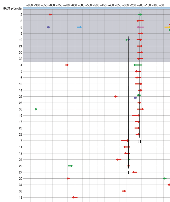
Figure 7. Composition of selected UAS elements from the HAC1 promoter tested in a wild-type strain. The selected fragments (colored arrows) are compared to the native promoter to reveal consensus regions. Numbering across the top represents the nucleotide position in the promoter relative to the start of translation. Arrow colors indicate the order of fragment assembly (5'-red-green-blue-purple-cyan-orange-3') and the arrow direction indicates a sense (pointing right) or antisense (pointing left) promoter fragment. The shaded gray encompasses clones with the strong phenotype. Two consensus region (I and II) are indicated with a vertical lines.
