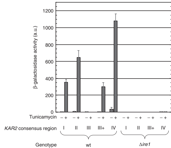
Figure 4. Quantitative \beta -galactosidase assays with the KAR2 consensus regions serving as UASs in the CYC1-lacZ construct. Multiple copies of regions I-IV, 3 \times , 2 \times , 3 \times and 4 \times respectively, were used in these constructs. Consensus region III and the extended region III (III + , Figure 3) were each analyzed. Assays were performed in wild-type (wt) and \Delta ire1 strains in the presence and absence of tunicamycin. \beta -Galactosidase activity is shown in arbitrary units and error bars represent 1 SD.
