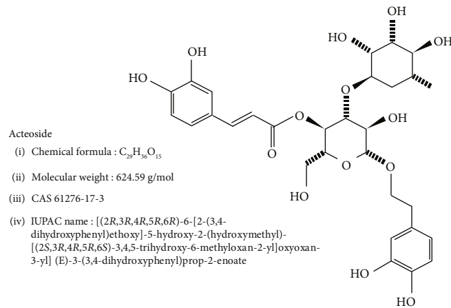
FIGURE 1: Chemical structure and information of acteoside.
