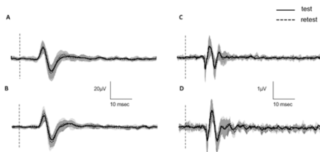
Figure 1. Representation of the grand average of VEMP results and standard deviation: A) cVEMP right ear; B) cVEMP left ear; C) oVEMP right ear; D) oVEMP left ear.
