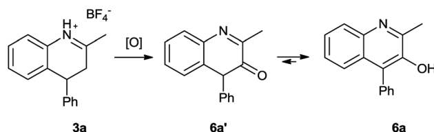
Scheme 4 Oxidation of dihydroquinoline 3a leading to 3-hydroxyquinoline.
